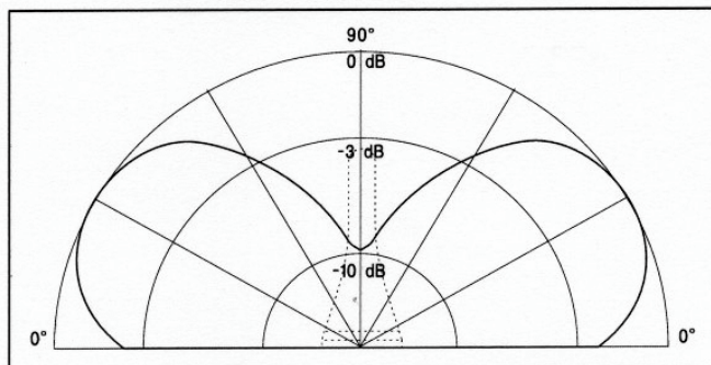
RADIATION PATTERN
